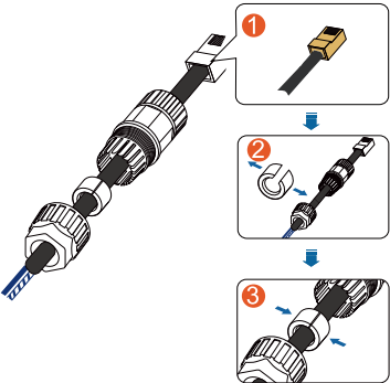
RJ45 terminal components (B)
